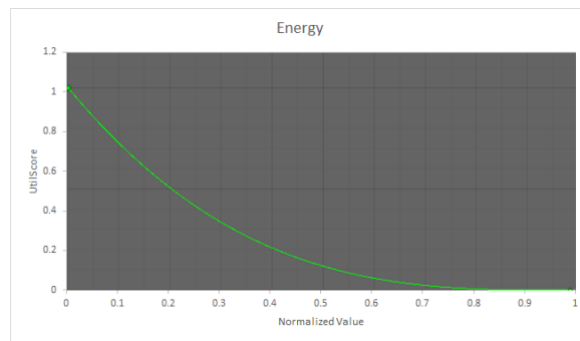
Figure 44: Energy Function for Run Away Action
