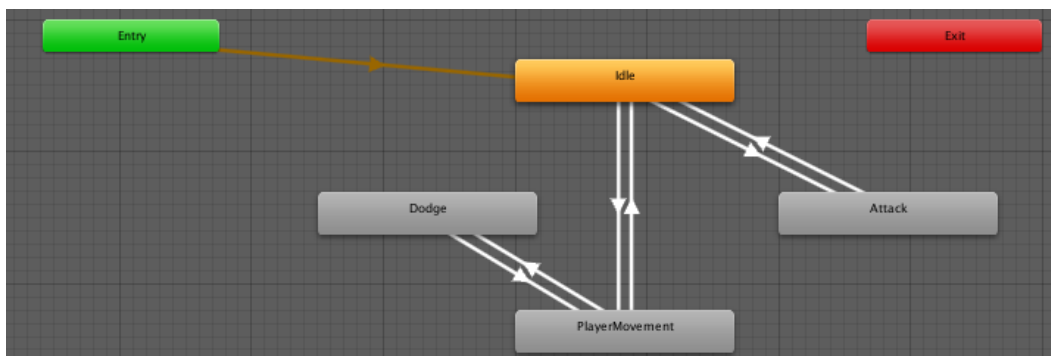
Figure 24: Animator Controller
