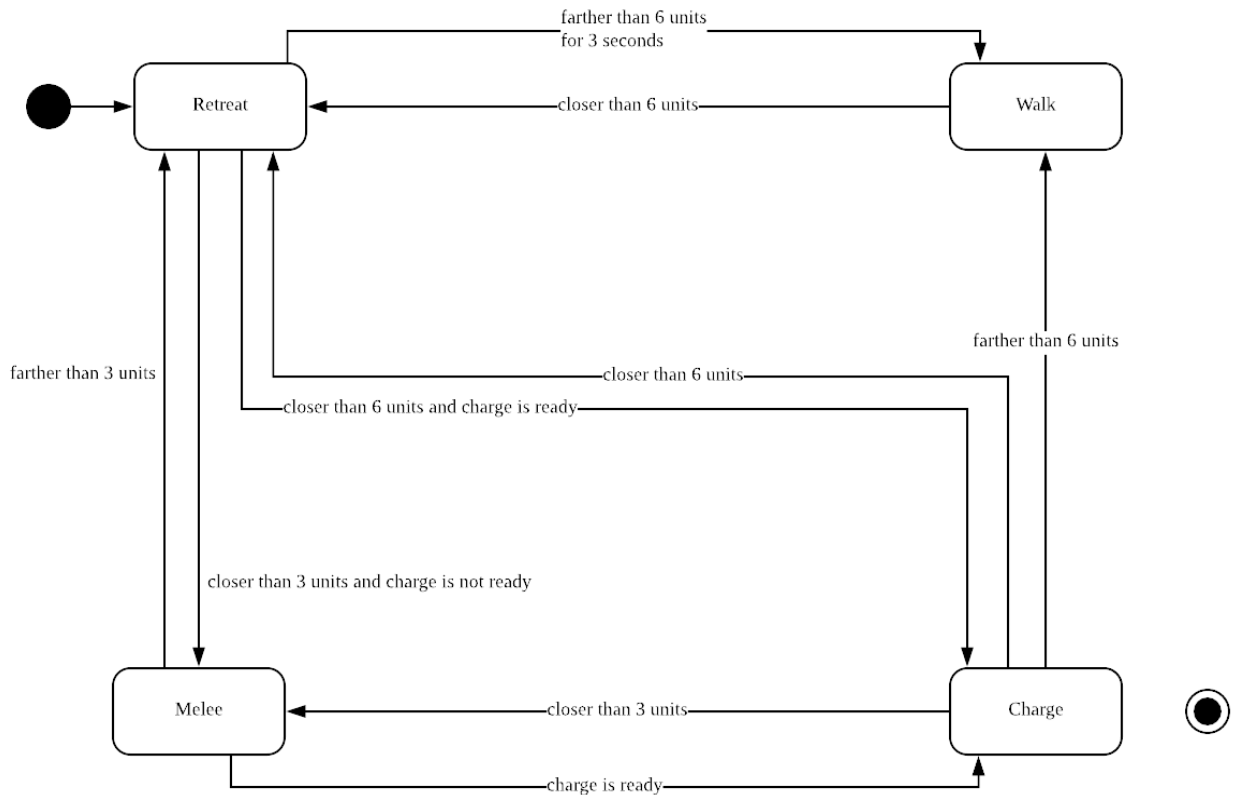
Figure 71: State diagram
