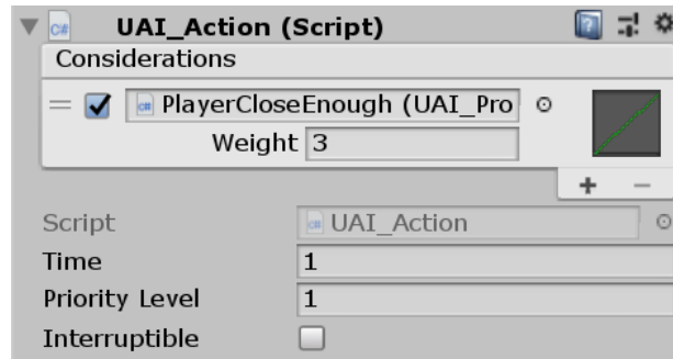
Figure 64: Melee action
