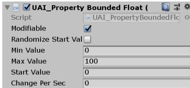
Figure 54: Tiredness property
