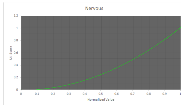
Figure 45: Nervous Function for Run Away Action
