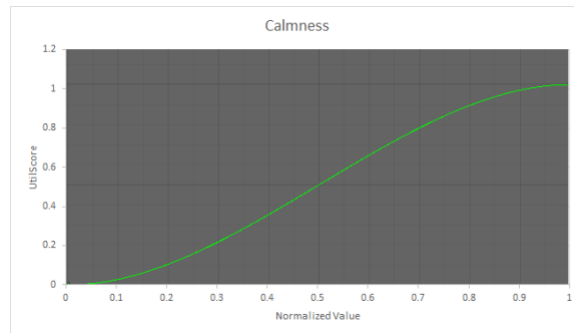
Figure 42: Calmness Function for Move Action
