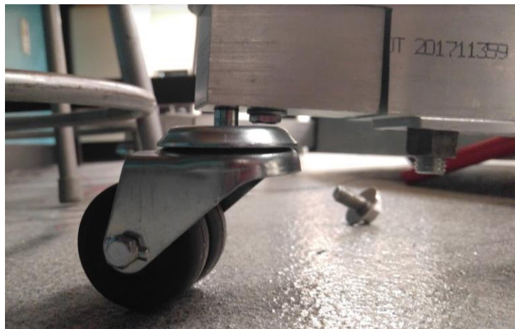
Figure 62: Back Wheel Connected to the Back Wheel Caster
