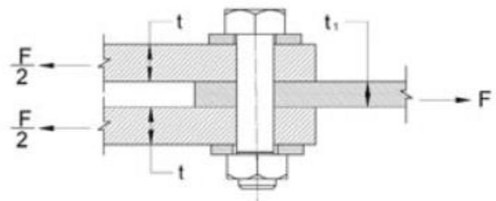
Figure 49: Pin Testing
