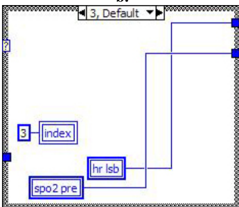
Figure B.3. Alternate cases for the read block (2).
