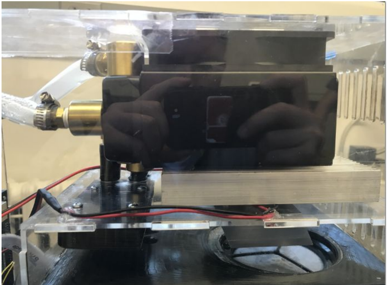
Figure 7: Radiator, Diffuser, Thermoelectric Cooler Assembly
