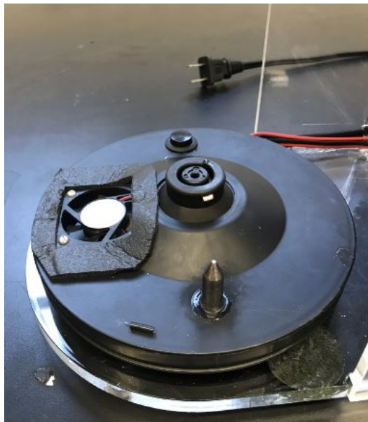
Figure 3: Kettle Base
