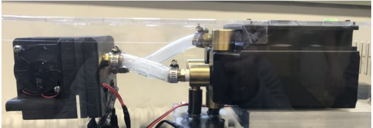
Figure 6: Vapor Blower Fans Output to Radiator Input
