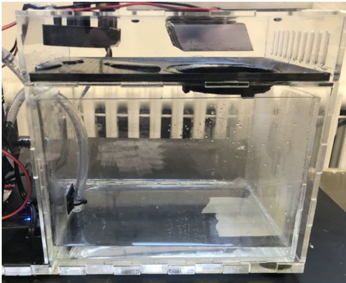
Figure 8: Sloped Surface, Filter, Collection Vessel Configuration
