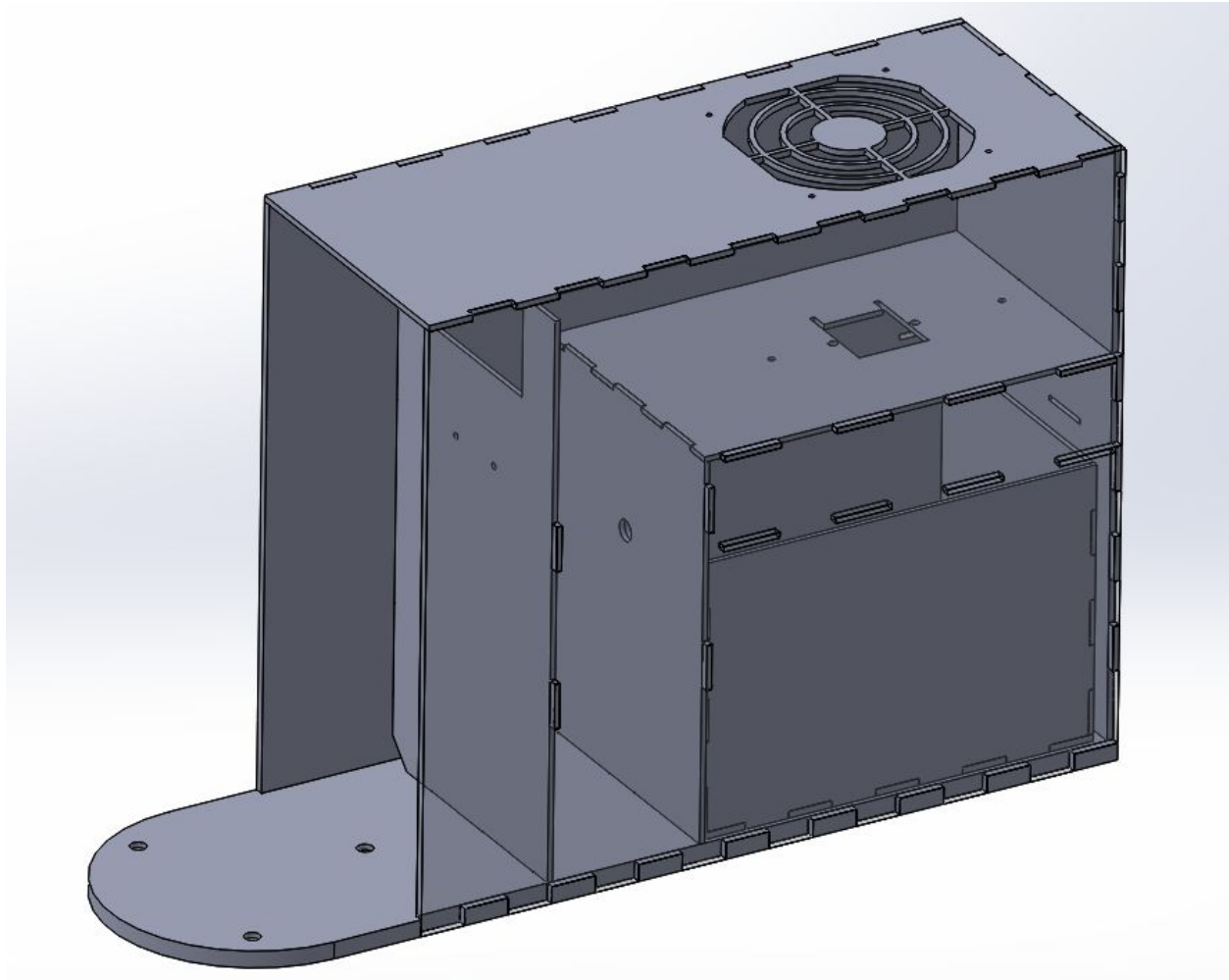
Figure 11: Solidworks Housing
