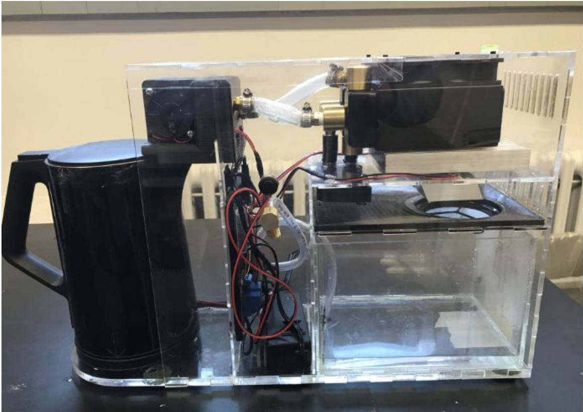
Figure 2: Full Prototype
