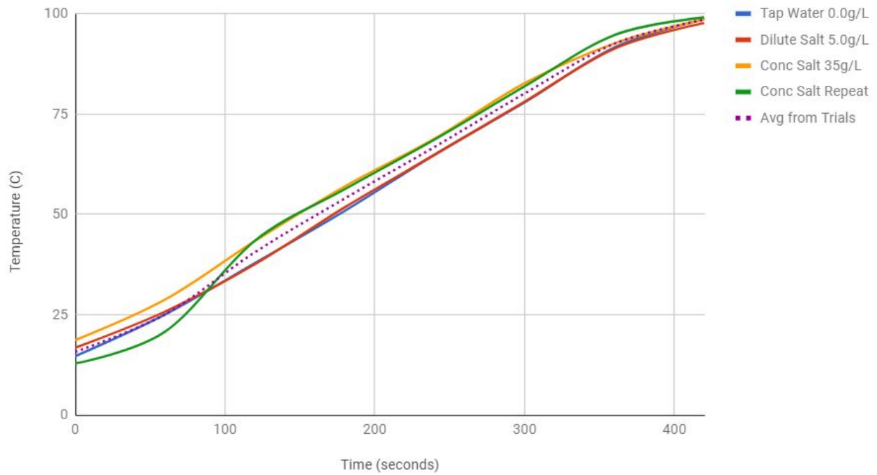
Temperature vs Time for Boiling of Water
