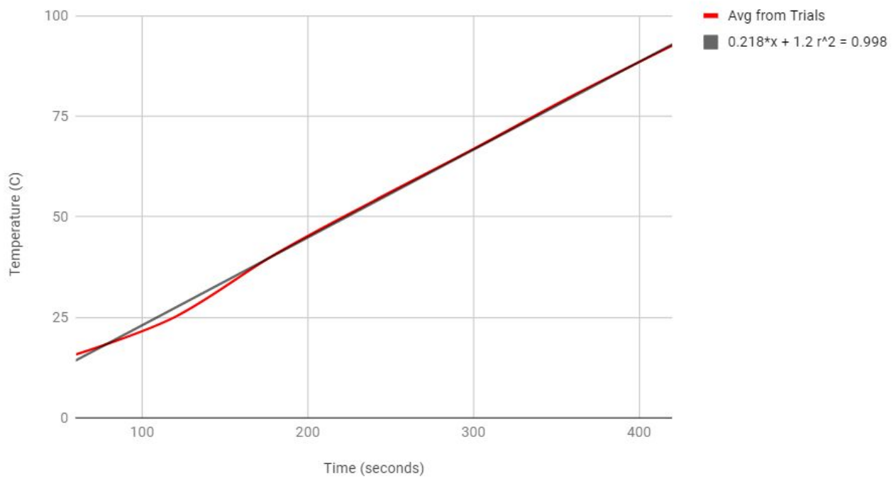
Average Temperature vs Time for Boiling
