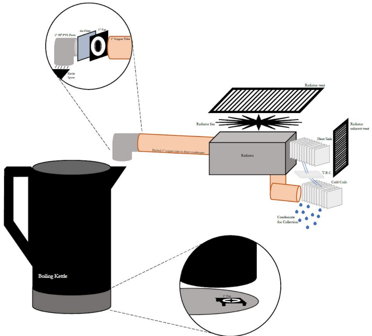
Figure 1: Operation Flowsheet
