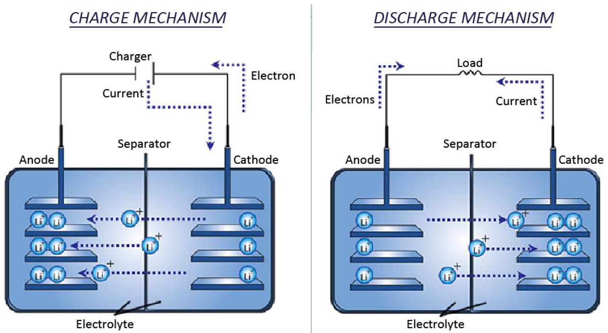
Figure 58 – Intercalation Cycle
