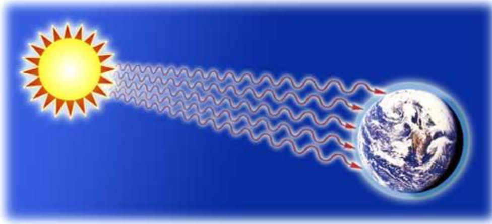
Figure 30 - The Sun's Radiation on Earth
