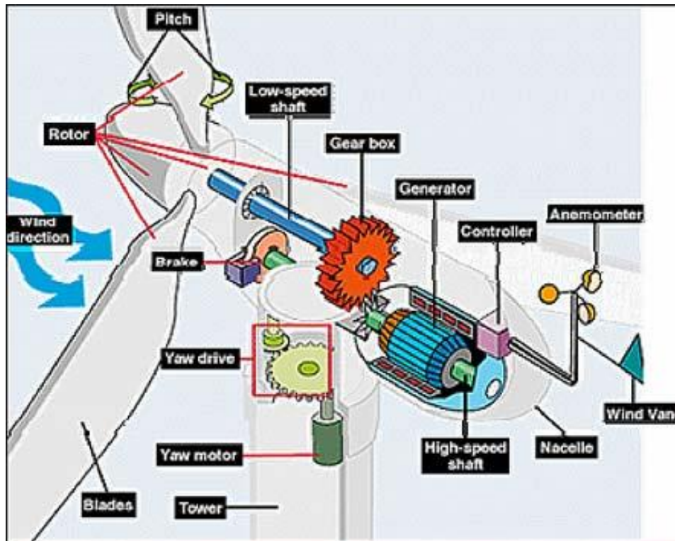
Figure 43 - Air Turbine Break-down [31]
