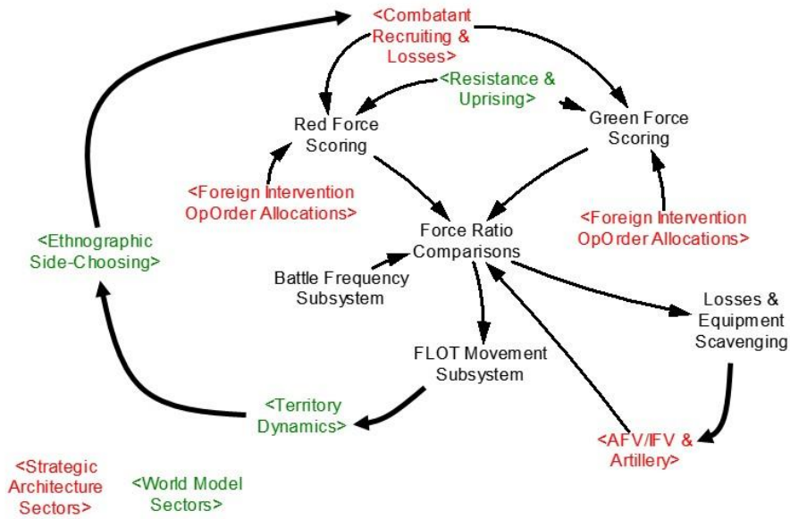
Figure D-11: Overview of SFS Combat Simulator Sector
