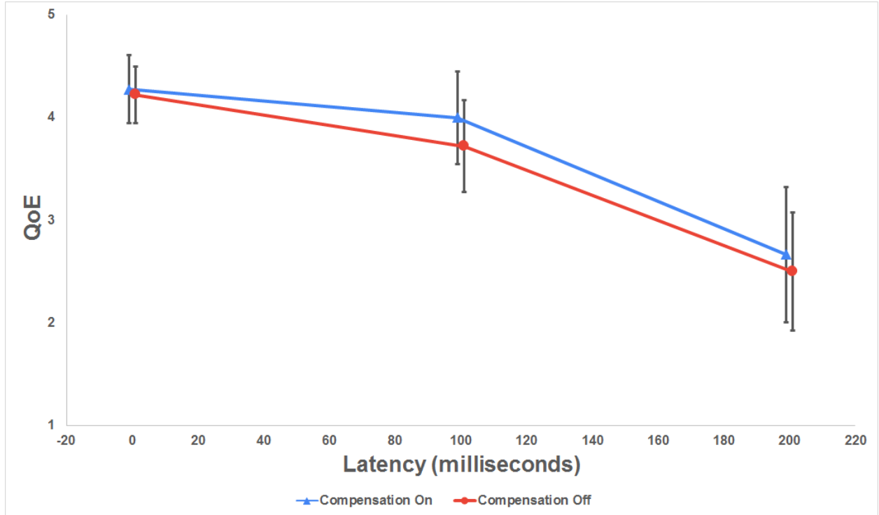
Figure 5.3.1: Average QoE (Quality of Experience) with Compensation on vs. Compensation off for each added latency category (0,100, and 200)
