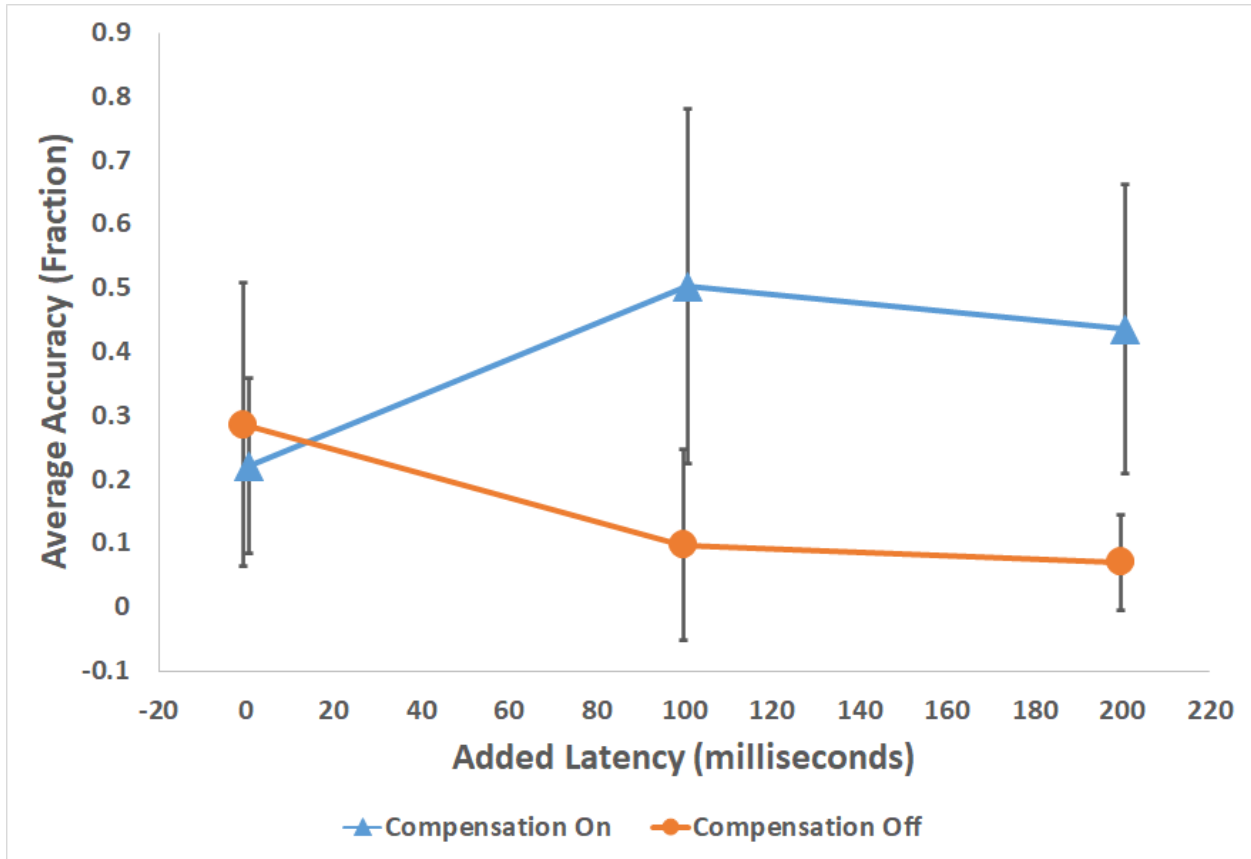
Figure 5.2.10: Lightning Strike Accuracy vs. Latency for Test Group
