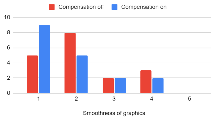
Smoothness of Graphics with 200 Added Latency
