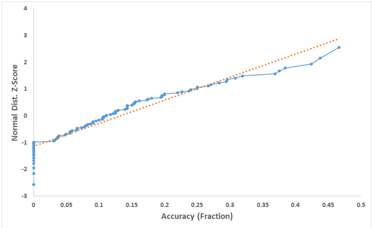
Figure 5.2.4: Quantile-Quantile Plot of Fireball Accuracies Across All Trials from Test Group
