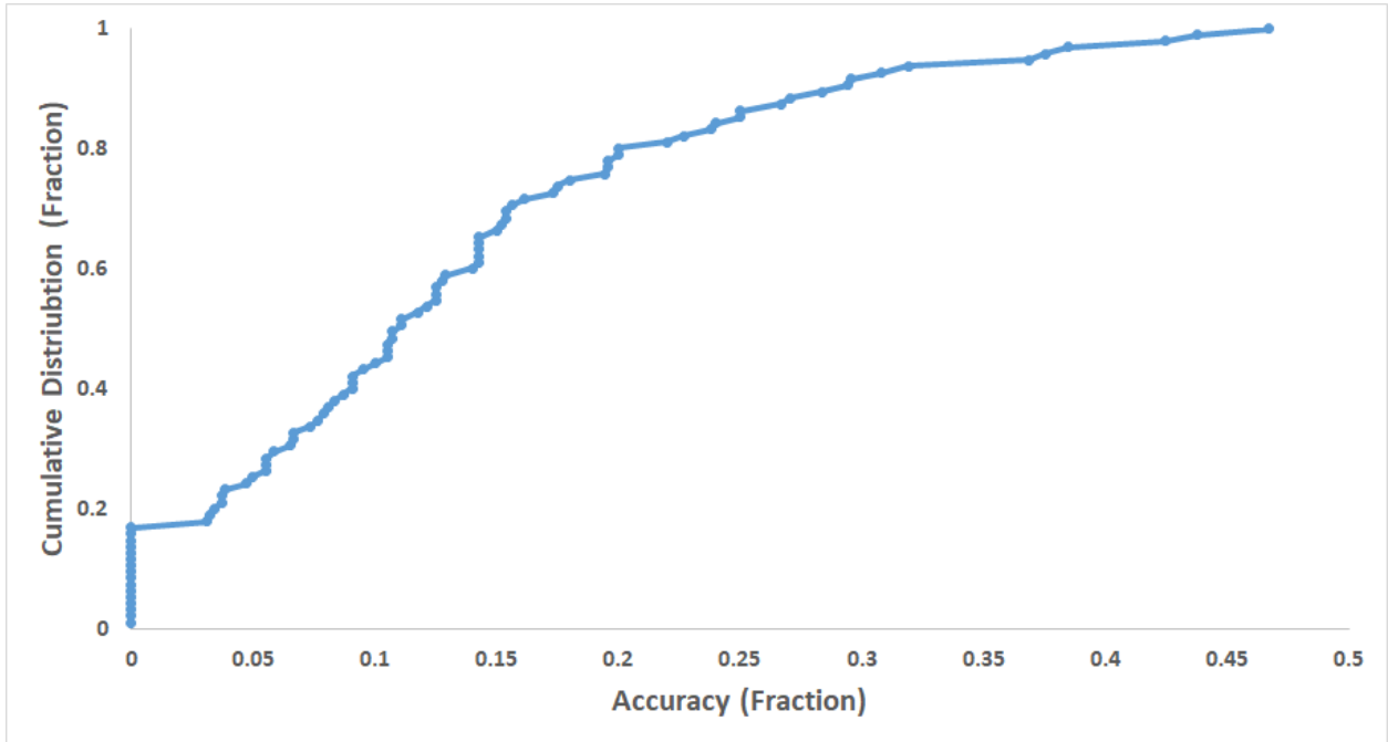
Figure 5.2.3: Cumulative Distribution of Fireball Accuracies Across All Trials from Test Group
