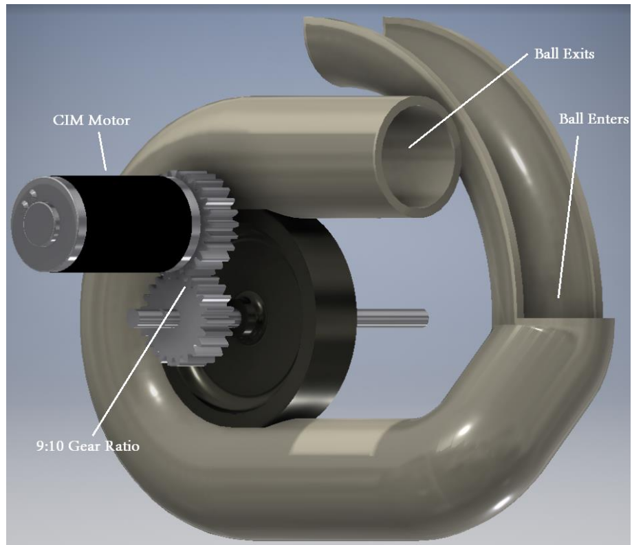
Figure 8: Launcher Design 2
