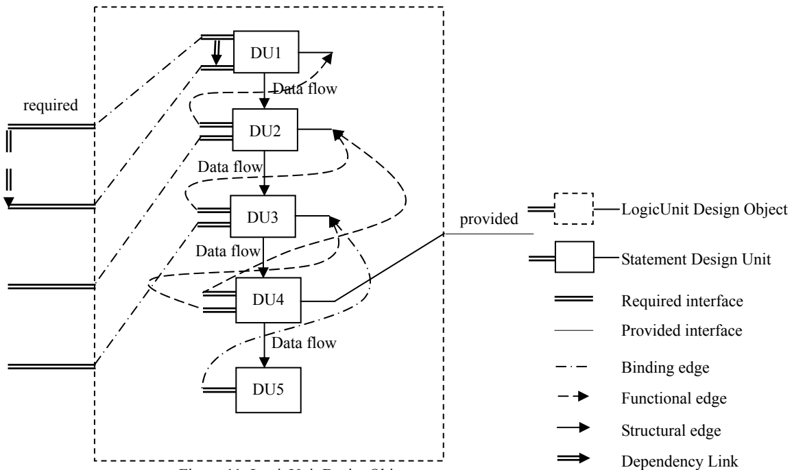
Figure 11: LogicUnit DesignObject
