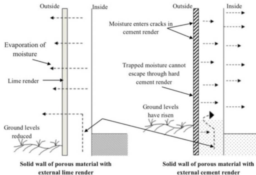
Figure 45: Visualization of the differences that lime and cement mortars have on moisture within a structure (roundtowerlime.com).
