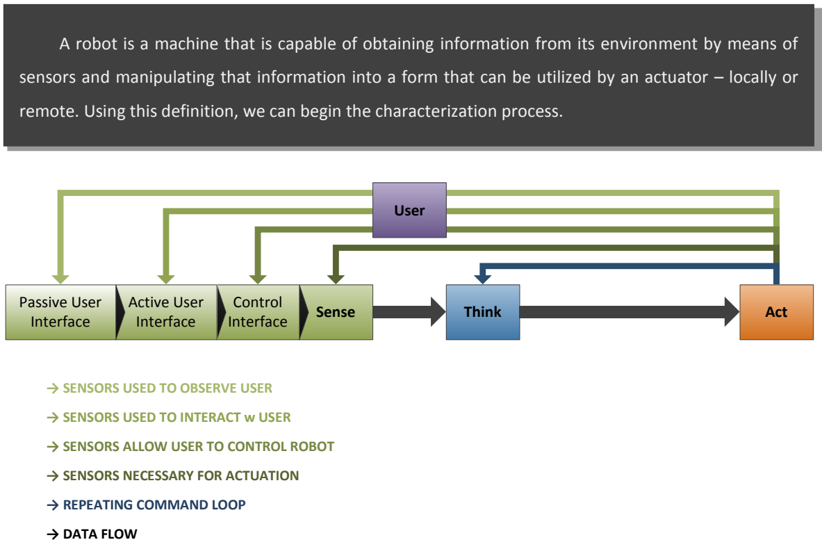
Figure 4.1.6 – Data Flow in Robot
