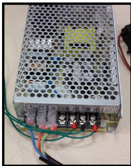
Figure 2.13 Power Supply
