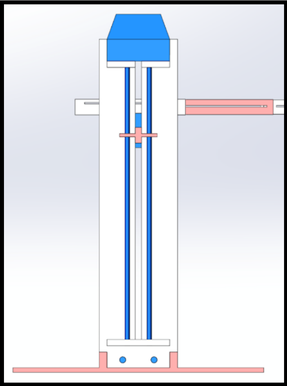
Figure 5.7 Side View
