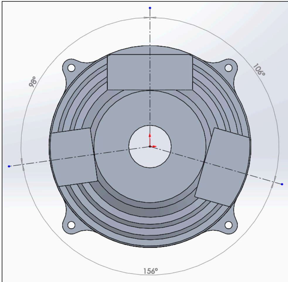
Figure 22: Cylinder shell port angles.
