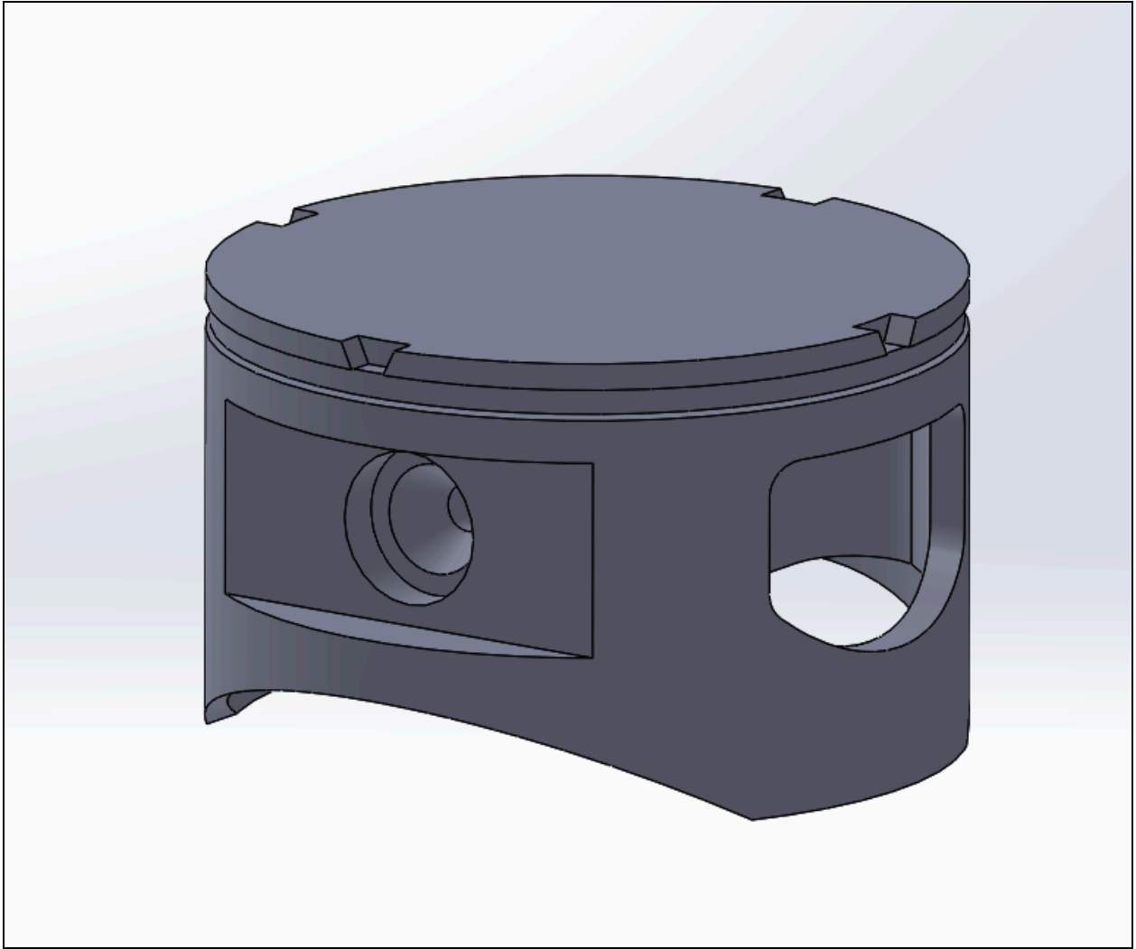
Piston Head with Ring and Wrist Pin
