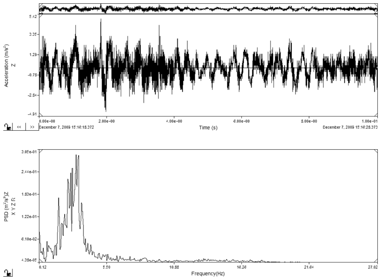
Figure 51: Secondary road , Ambulance #3, Z-Axis R.M.S., \leq 35 - 64 mph., typical 10 sec event interval
