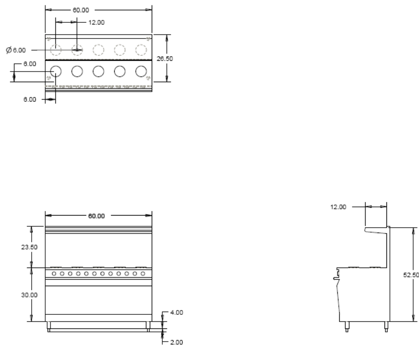
Figure 20: Top, Front, and Side Views of Range
