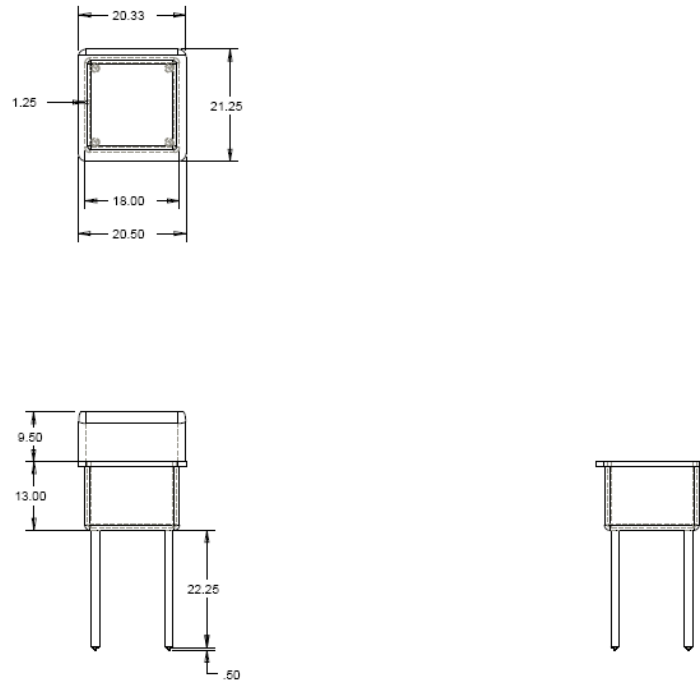
Figure 22: Top, Front and Side Views of Sink
