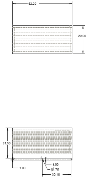
Figure 18: Top, Front, and Side Views of Generator
