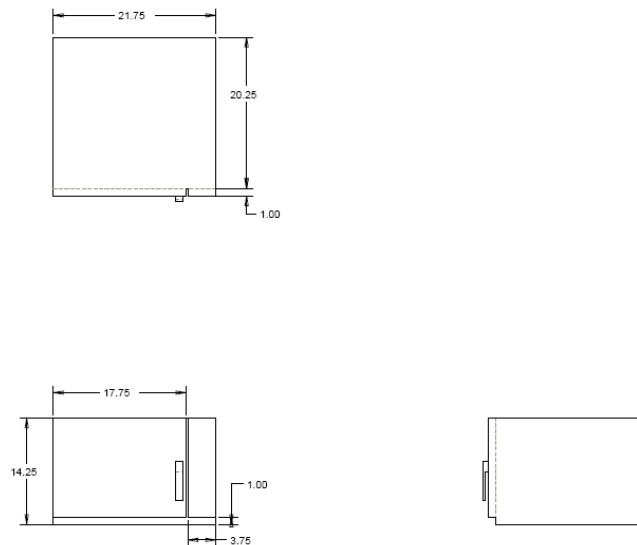
Figure 19: Top, Front and Side Views of Microwave
