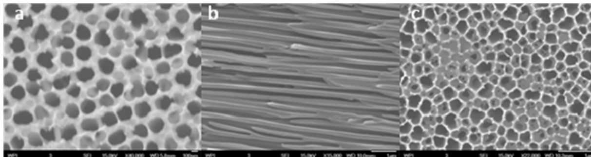
Fig.3 a) Top view of an empty AAO template; b) Cross-sectional view of an empty AAO template; c) Top view of BSA multilayers deposited inside AAO template. (The scale bars are a) 1 \mu m; b) 100 nm; c) 1 \mu m)
