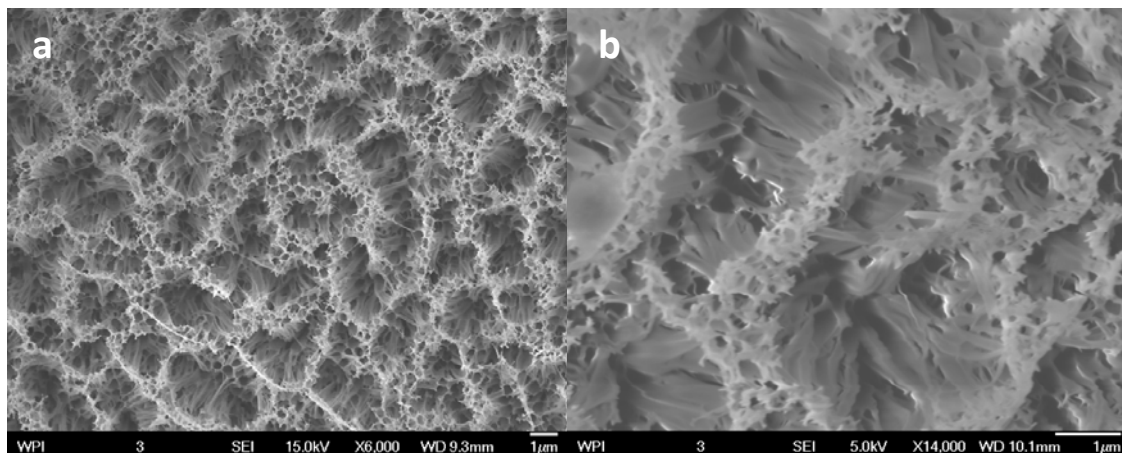
Fig. 4 SEM images of AAO template after etching with 5% \text{H}_3\text{PO}_4 for 16 hours
