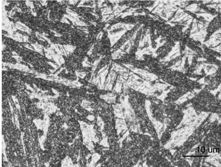
Figure 44: Microstructure of forged 4140 steel blade.
