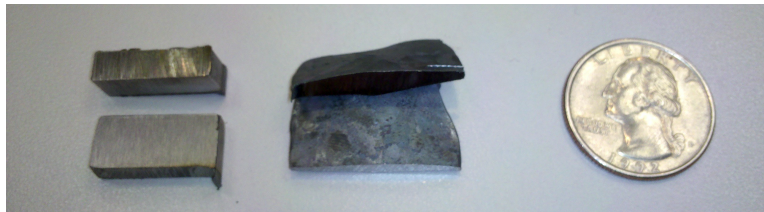
Figure 20: The steel samples with quarter for scale. Left: Unforged steel. Middle: Heated and shaped steel.
