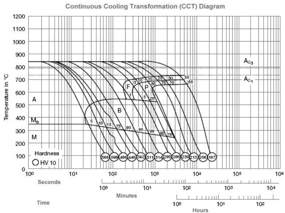
Figure 45: CCT diagram (website: "42CRMOS4").
