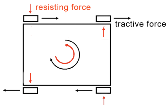
Figure 18 - Skid Steering
