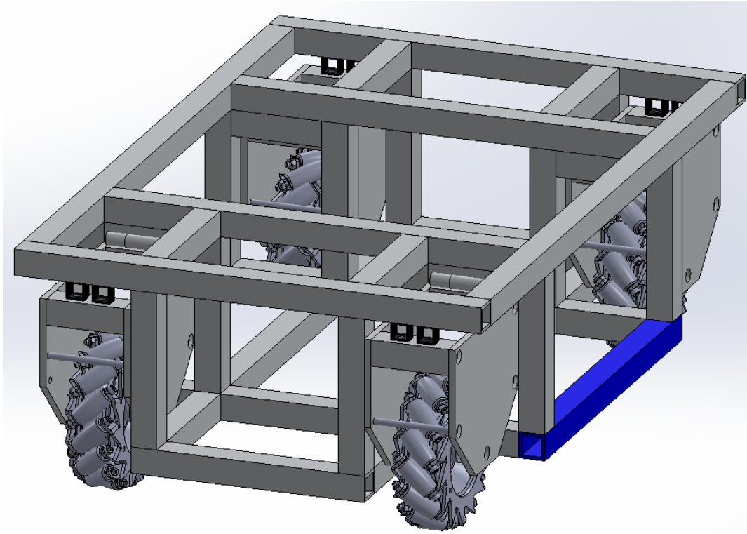
Figure 20: Chassis Design
