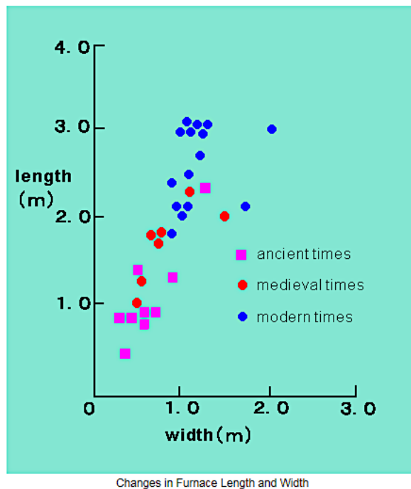
FIGURE 20. VARIATIONS IN SIZE OF THE TATARU FURNACE (“ABOUT TATARU” 1).
