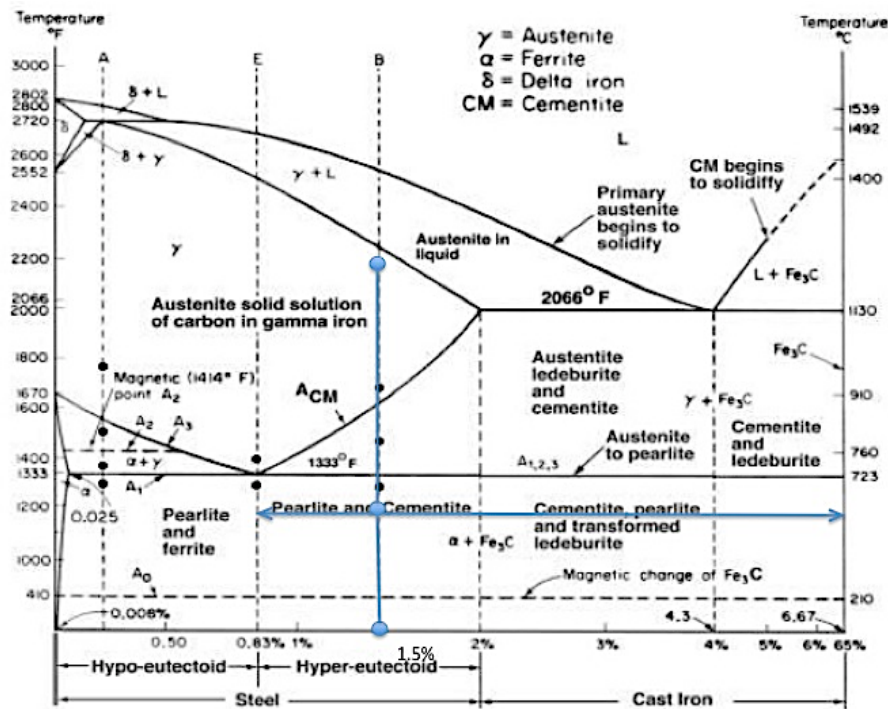
FIGURE 27. FE 3 C PHASE DIAGRAM WITH CALCULATIONS.
