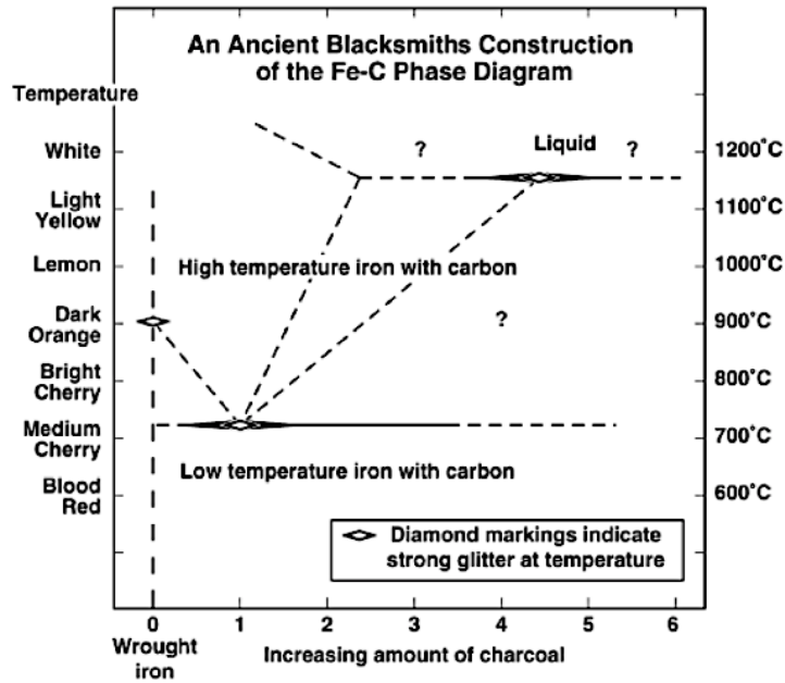
FIGURE 10. A HISTORICAL BLACKSMITH Fe_3C PHASE DIAGRAM.
