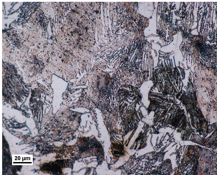
FIGURE 50. X AXIS OF SAMPLE AT 20X.
