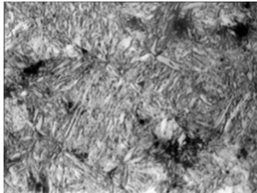
FIGURE 28. MARTENSITE MICROSTRUCTURE.
