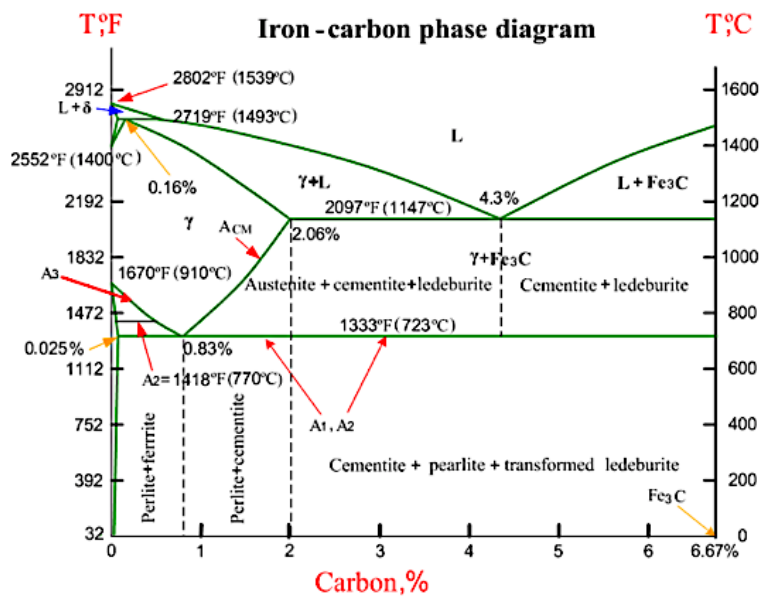
FIGURE 11. A MODERN Fe_3C PHASE DIAGRAM.
