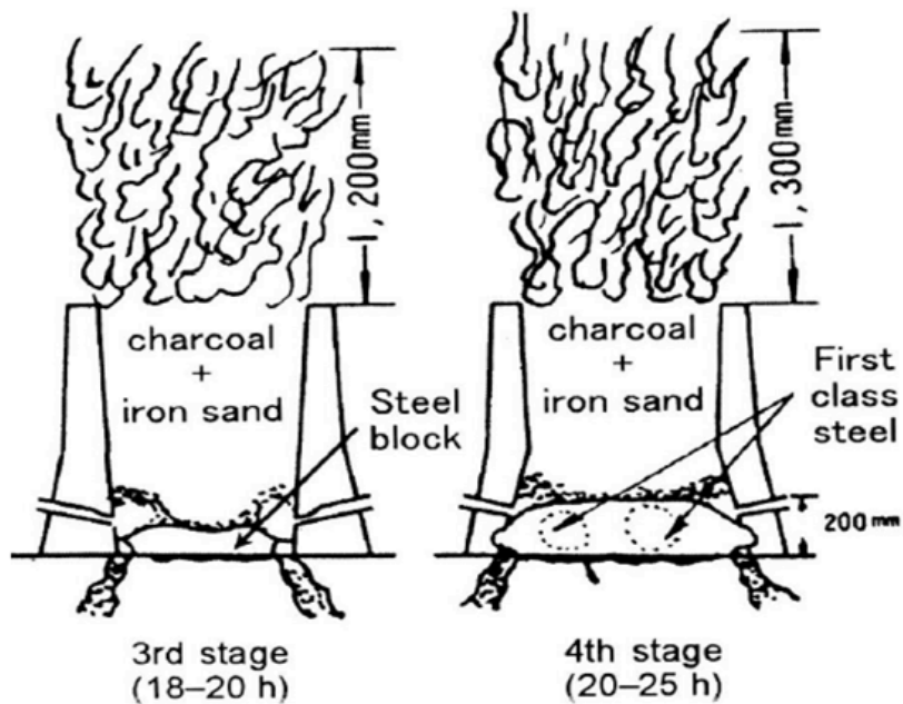
FIGURE 18. TATARA FURNACE STAGES 3 AND 4 (KITAMURA 278).
