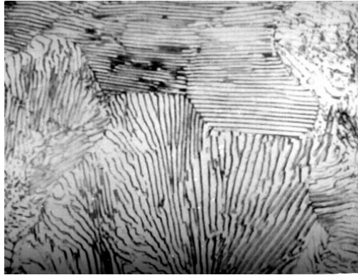
FIGURE 29. PEARLITE MICROSTRUCTURE.
