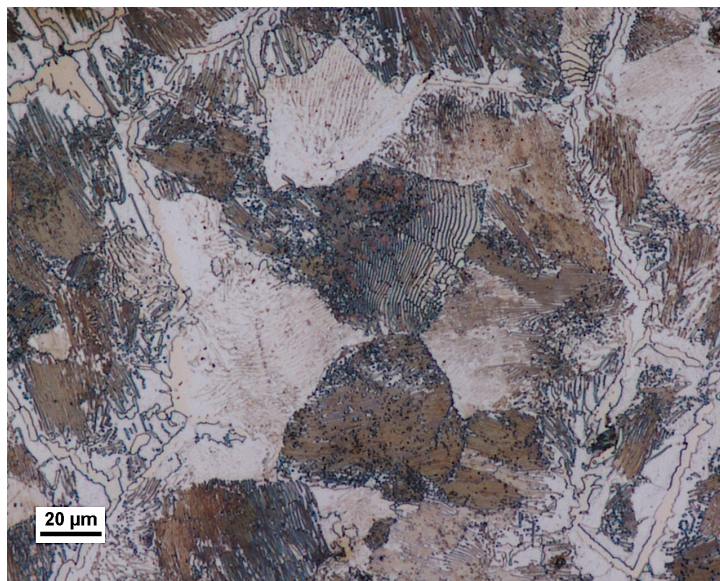
FIGURE 52. Z AXIS OF SAMPLE AT 20X.
