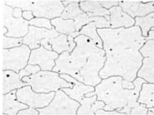
FIGURE 31. FERRITE MICROSTRUCTURE.
