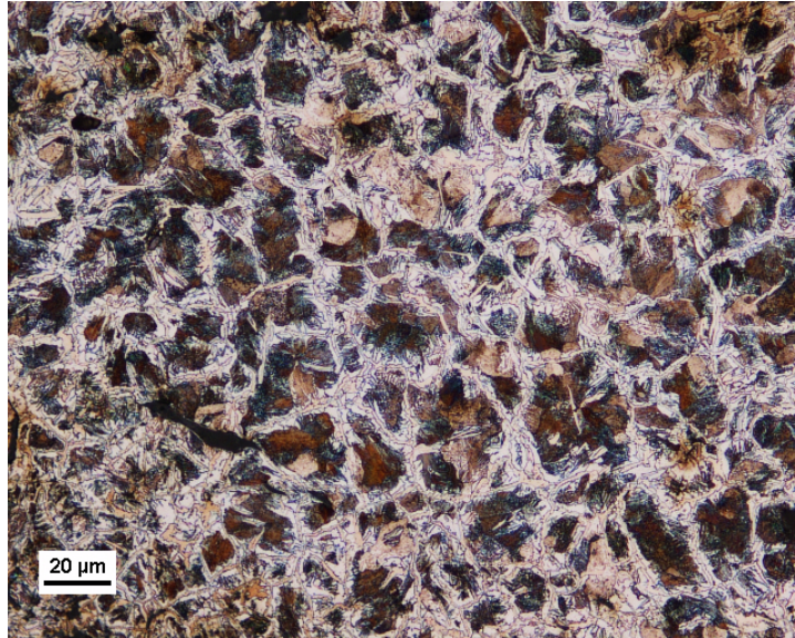
FIGURE 48. Y AXIS OF SAMPLE AT 20X.
