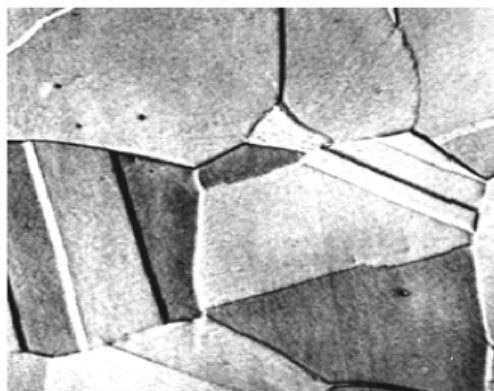
FIGURE 30. AUSTENITE MICROSTRUCTURE.
