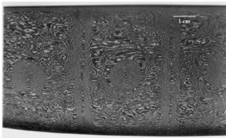
FIGURE 7. CARBIDE PATTERNS IN DAMASCUS STEEL.
