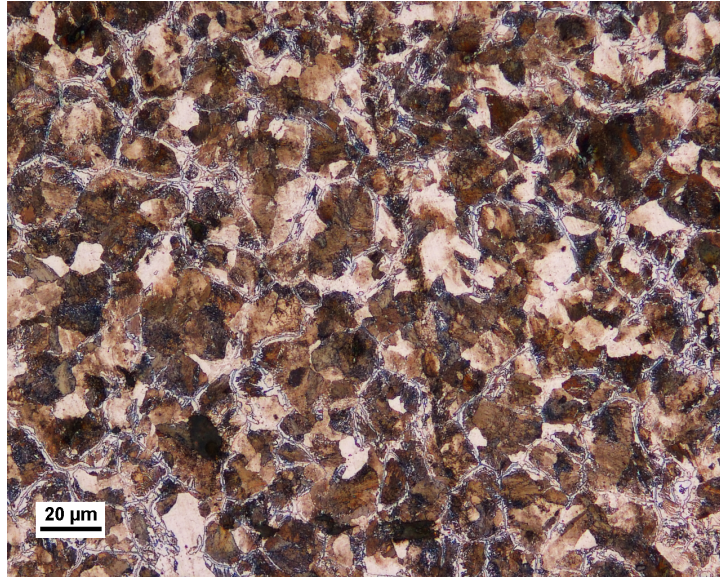
FIGURE 52. Z AXIS OF SAMPLE AT 20X.
