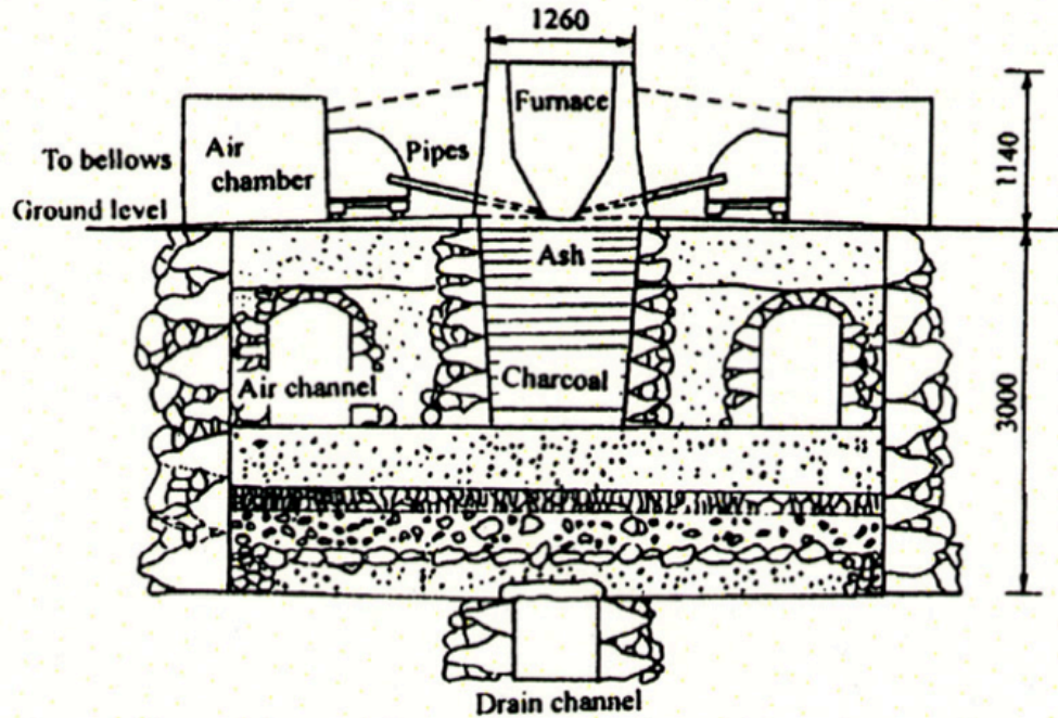
FIGURE 14. A TATARU FURNACE (INOUE 194).
