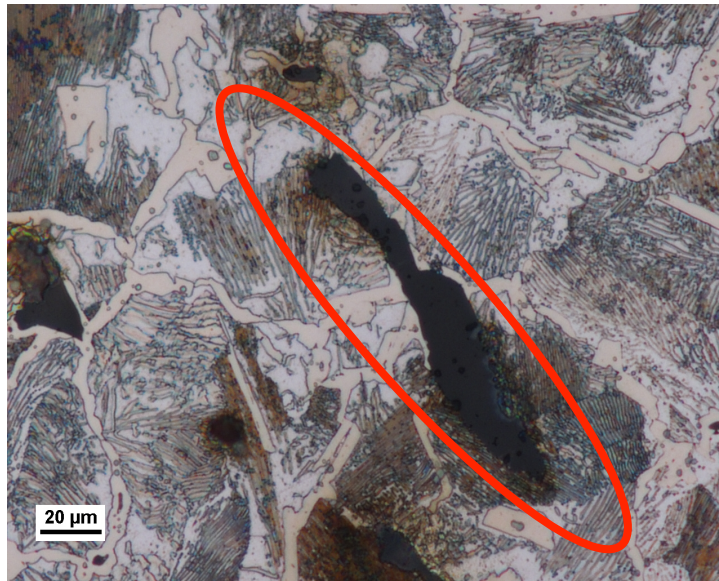
FIGURE 54. SLAG INCLUSION IN THE XZ FACE.
