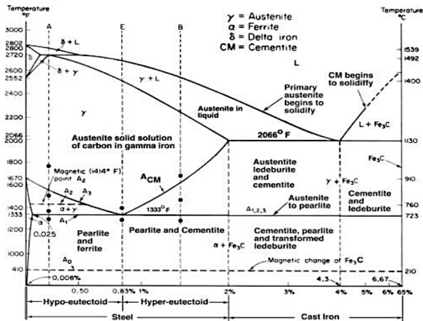
FIGURE 25. FE- \text{Fe}_3\text{C} PHASE DIAGRAM.
