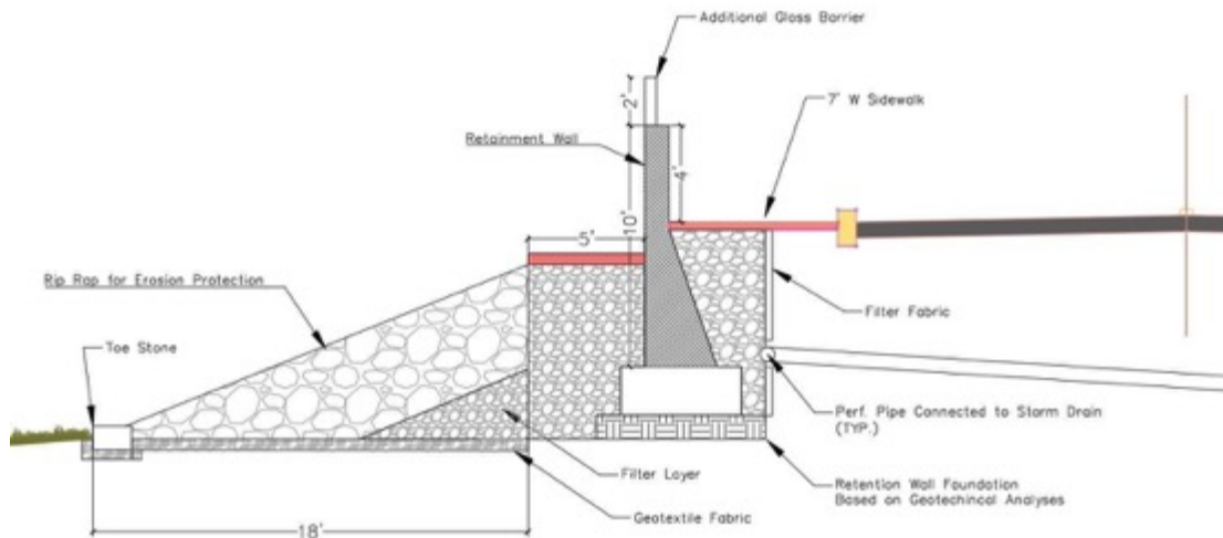
Figure 43. CAD Drawing - Replaced Wall, Rock Revetment, Extended Urban Wild Walkway
