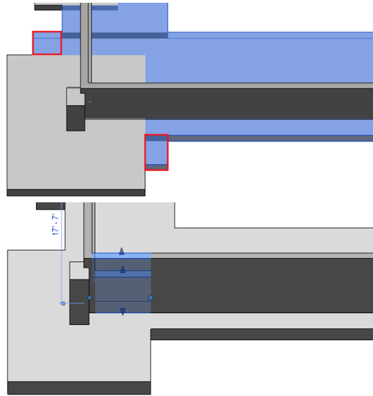
Figure 22 - Eccentric Continuous Footings
