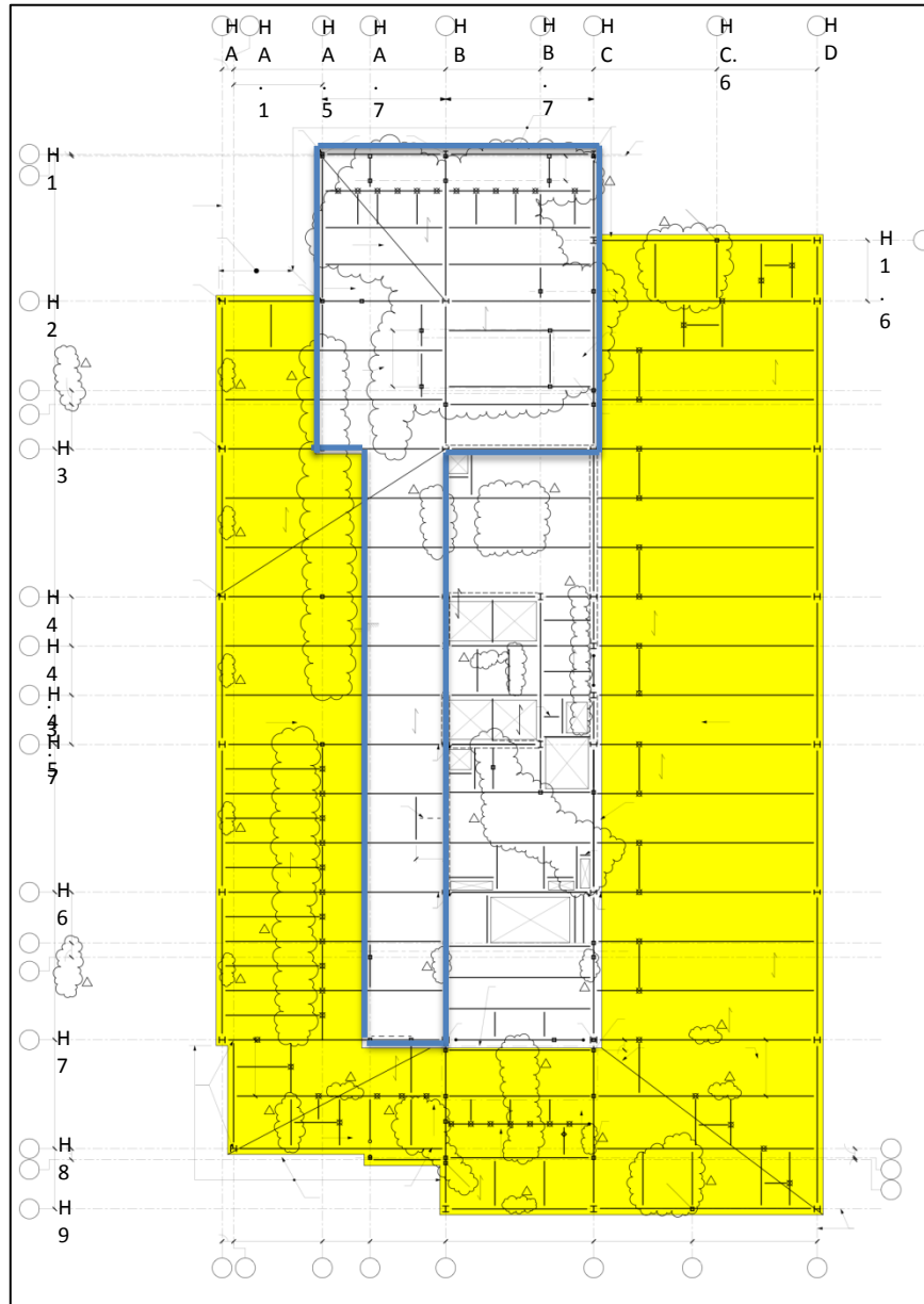
Figure 27 - Roof Floor Plan
