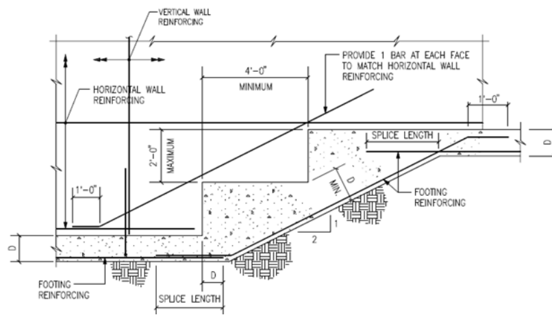
Figure 20 - Typical Detail at Continuous Stepped Wall Footing
