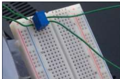
Figure 22: R2 Replaced with 1000Ω Potentiometer
