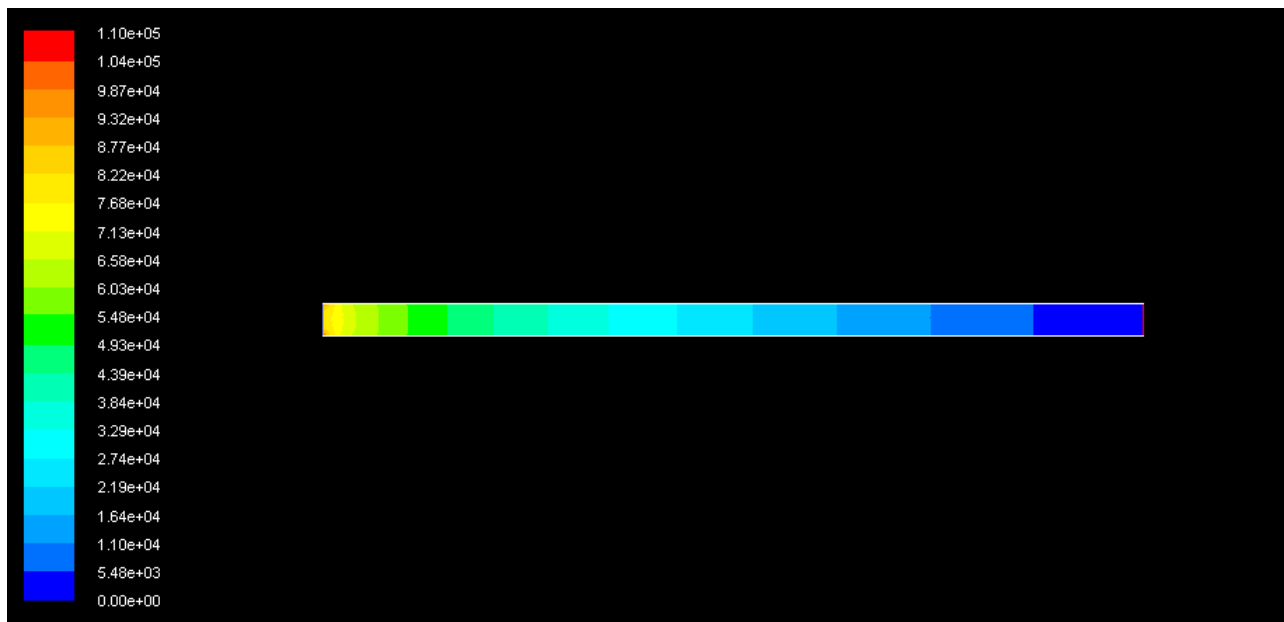
Figure 34: Pressure profile of multiphase flow in 10cm empty channel
