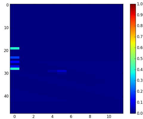
Figure 5.17: Predicting Restroom using Office and Restroom, BIC = 2120
