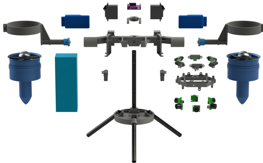
Figure 4.1: A CAD rendering of the TRo aircraft.
