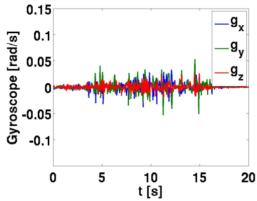
(b) Gyroscope data with fans at idle
