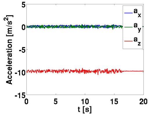
(b) Acceleration data with fans at idle
