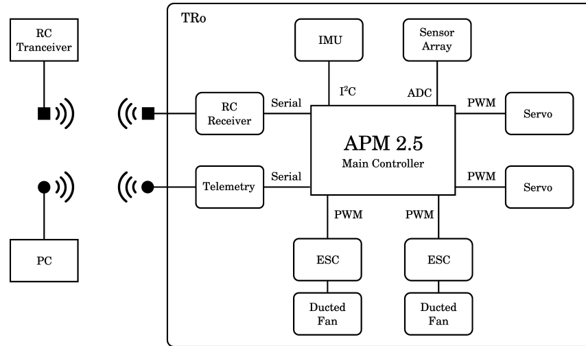
Figure 4.8: The electronics block diagram of the full scale tiltrotor.
