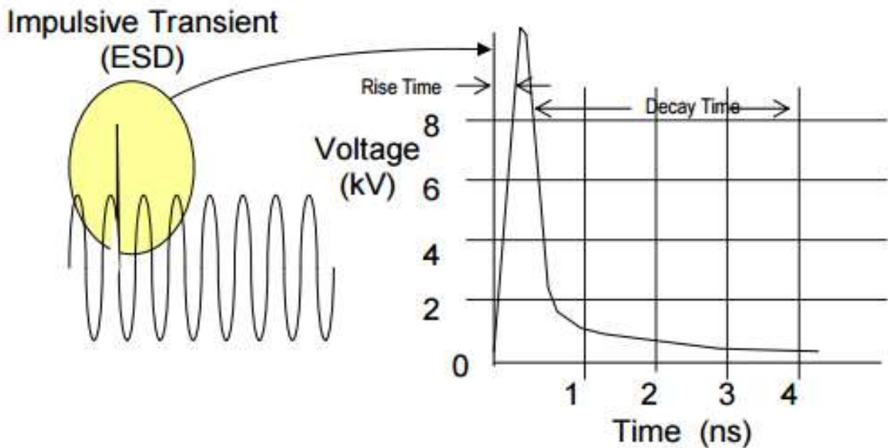
Figure 20. Impulse Transient 53
