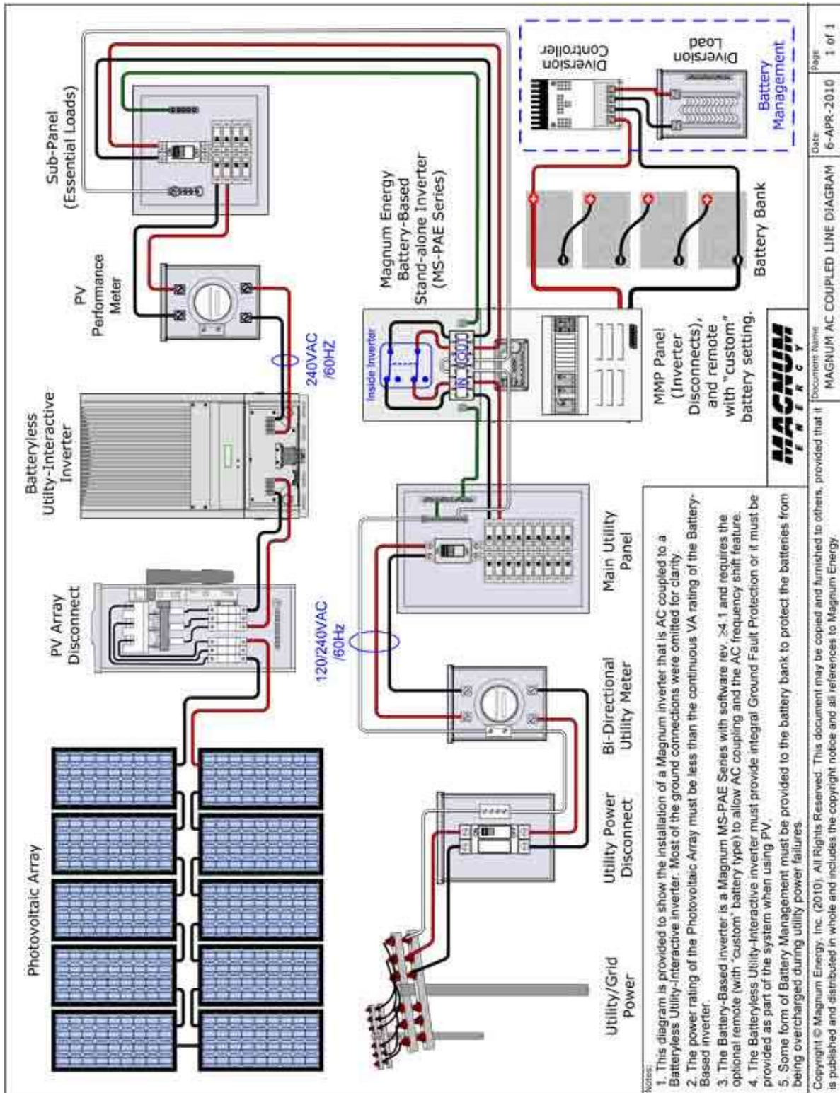
Figure 9. A Grid-tie System with Battery Backup 24
