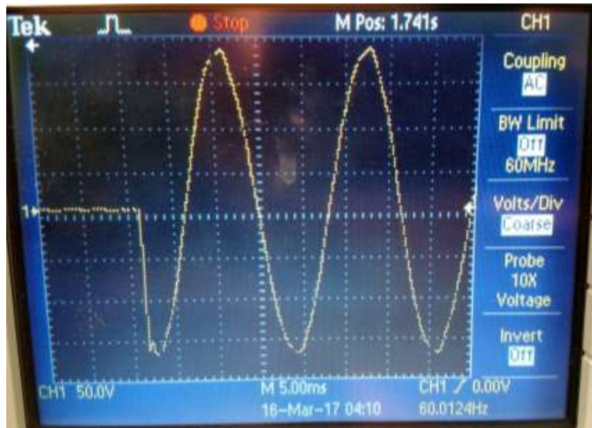
Figure 50. Electronic Breaker Transient Testing - Breaker Closing and Restoring Power
