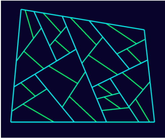
Figure 46 - Sample of a the grammar based subdivision output using 5 iterations
