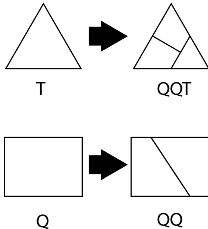
Figure 45 - Example of how grammar based subdivision works
