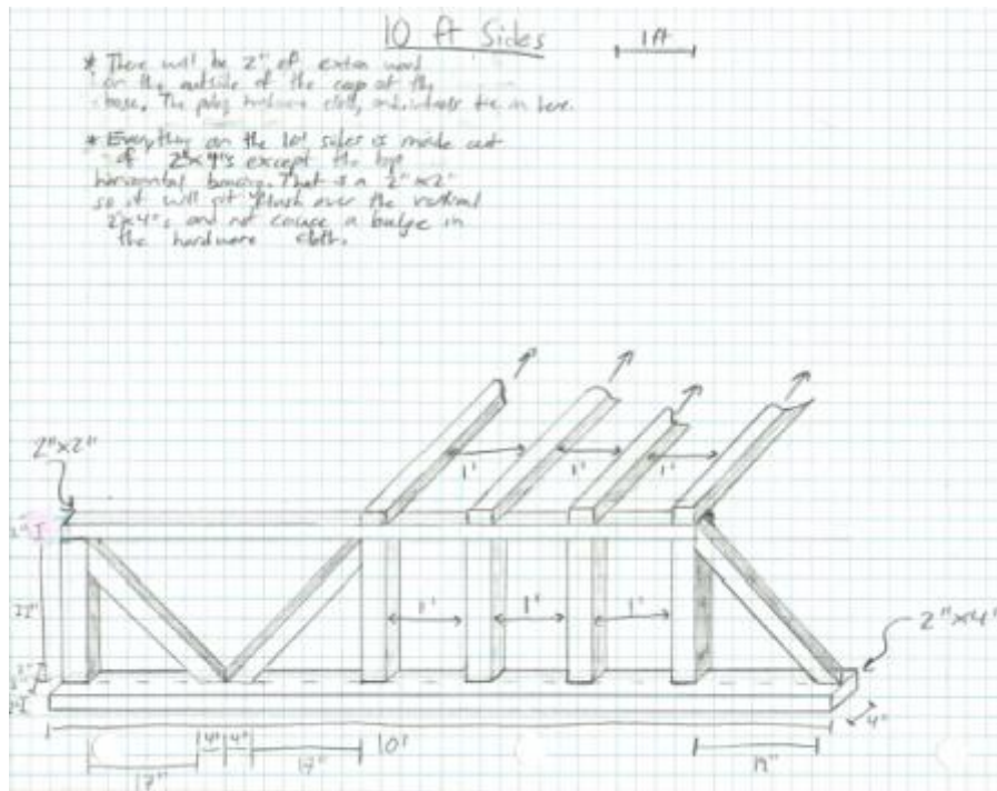
Figure 84: Hoop Coop Sketch Side View
