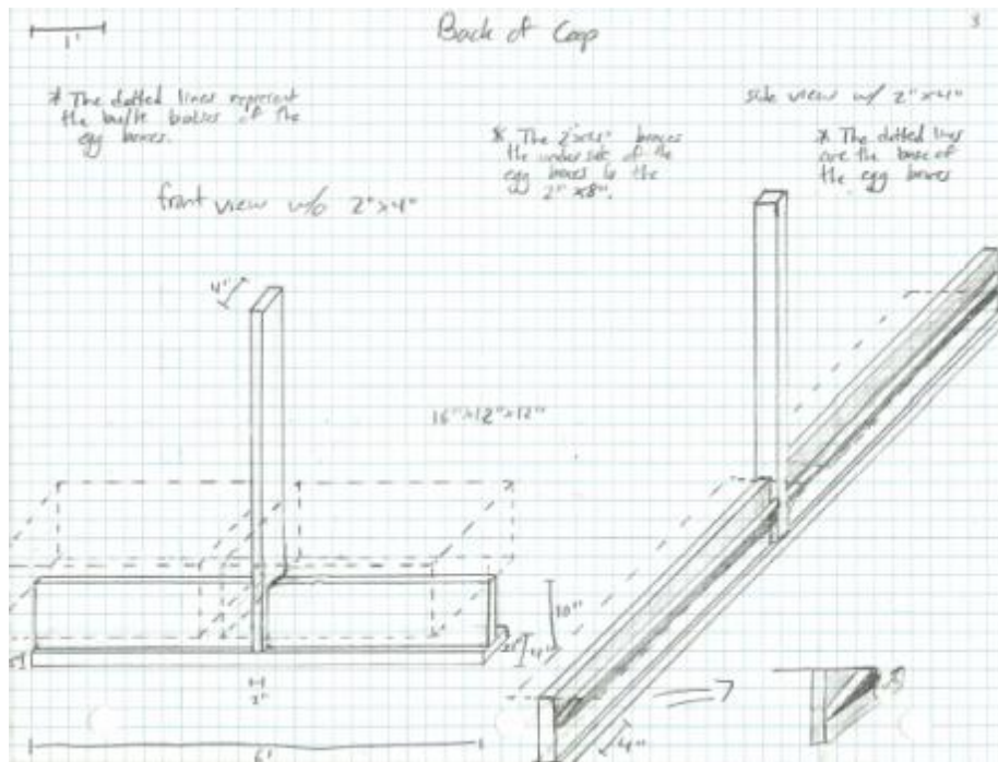
Figure 83: Hoop Coop Sketch Back View
