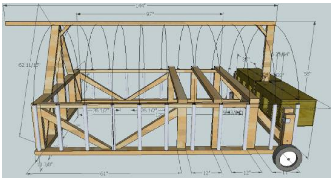
Figure 6: Hoop coop design
