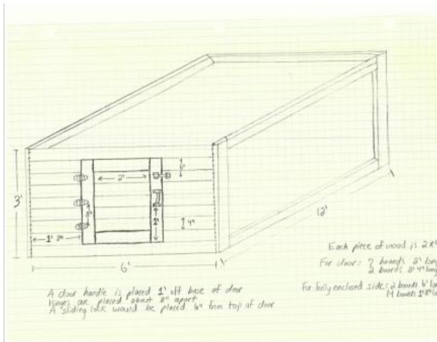
Figure 89: Hybrid Hoop Coop Sketch Door
