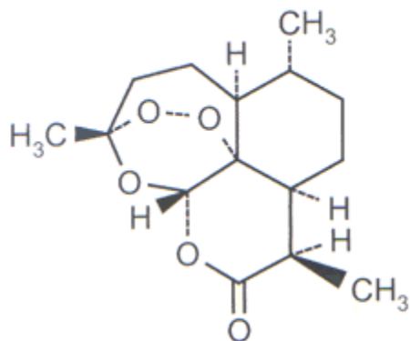
Figure 1.2. Structure of artemisinin.
