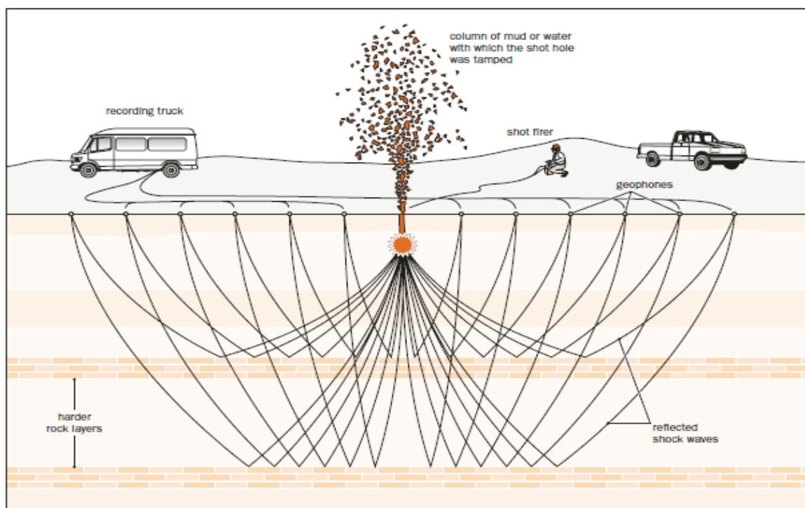
Figure 5: Seismic Testing
