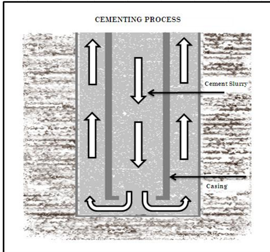
Figure 18: Cementing Process
