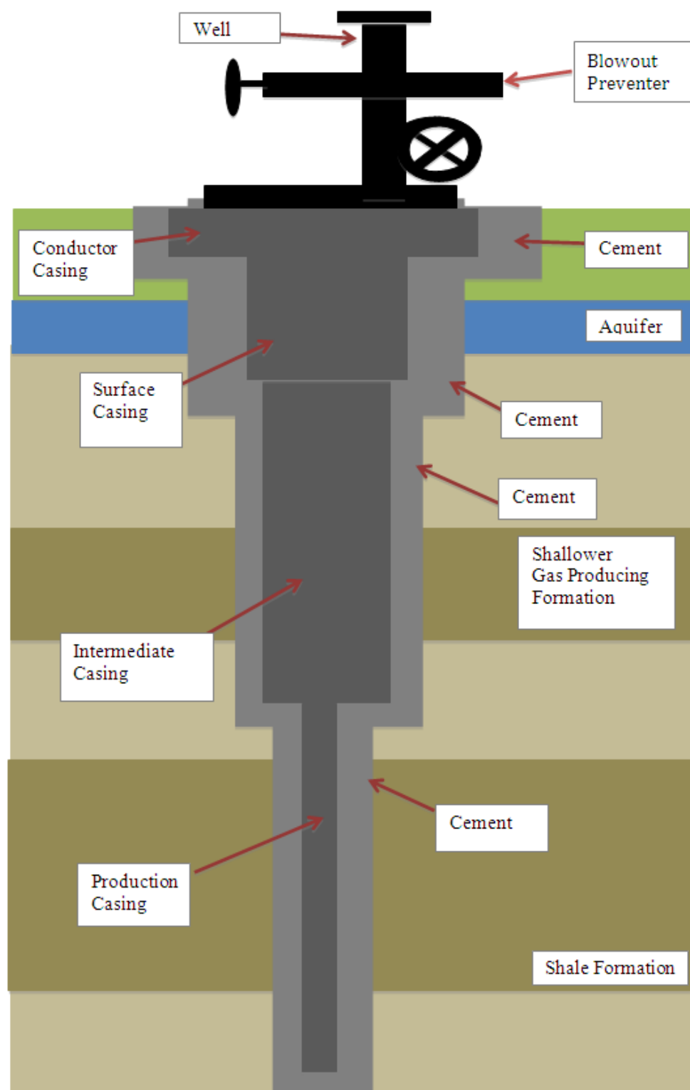
Figure 26: Well Diagram
