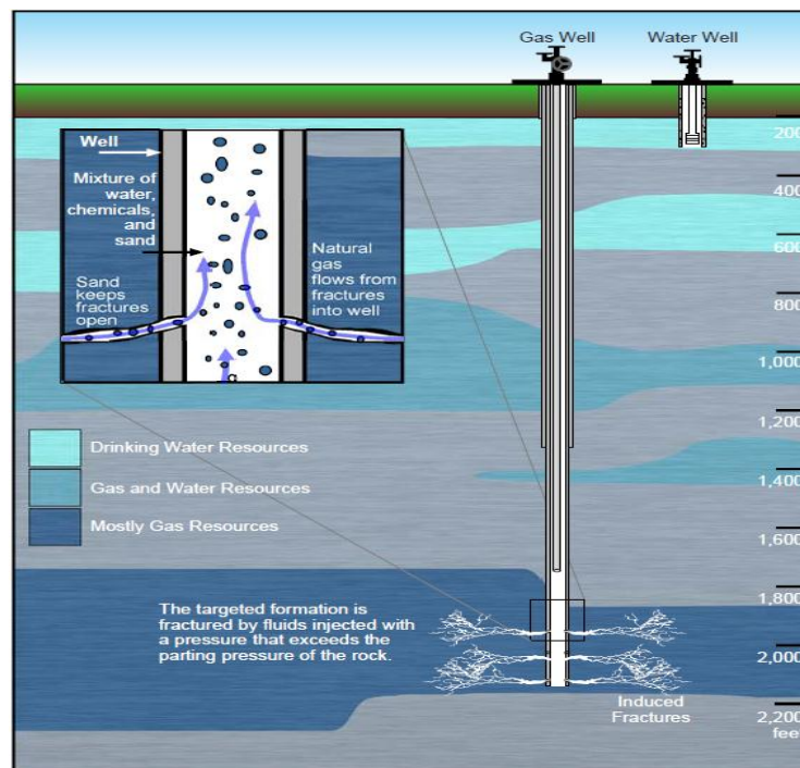
Figure 8: Vertical Well Construction
