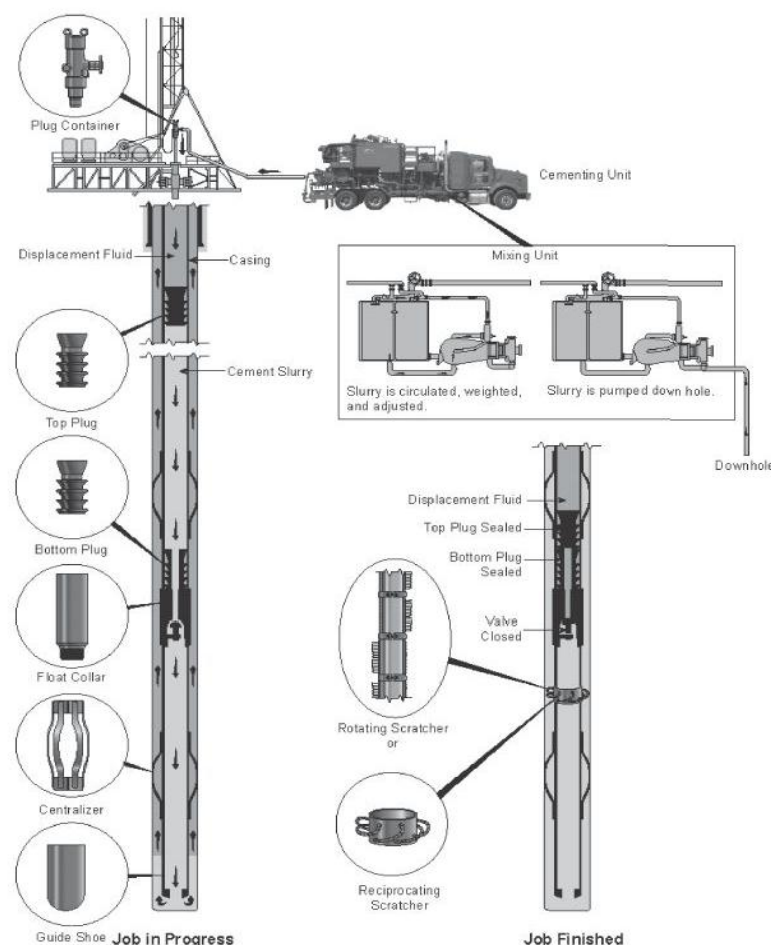
Figure 20: Cementing Process
